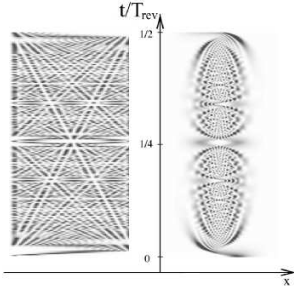
Figure 10: The quantum carpets for the Pöschel-Teller and Rosen-Morse potentials [85].
