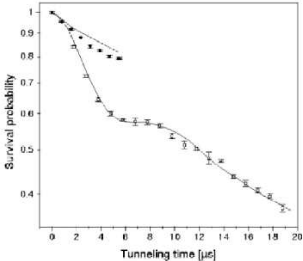
Figure 1: Observation of the Quantum Zeno Effect in the experiment [33].
