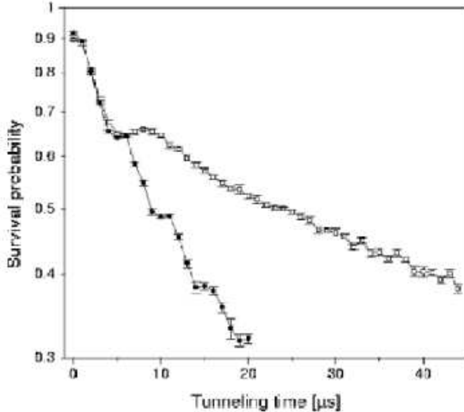
Figure 2: Observation of the Quantum Anti-Zeno Effect in the experiment [33].
