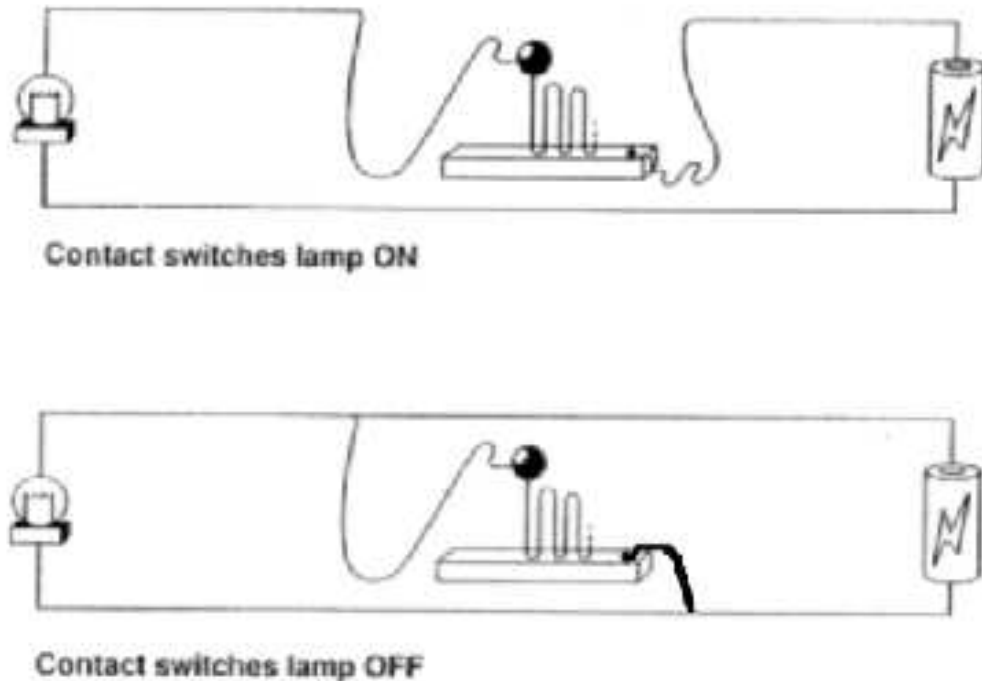
Figure 4: Alternative switching mechanisms for Thomson’s lamp from [42].
