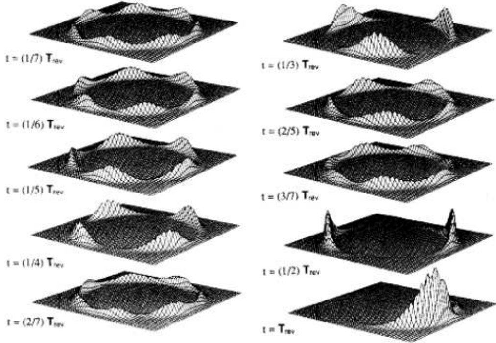
Figure 9: Wave-packet revival and fractional revivals [82].
