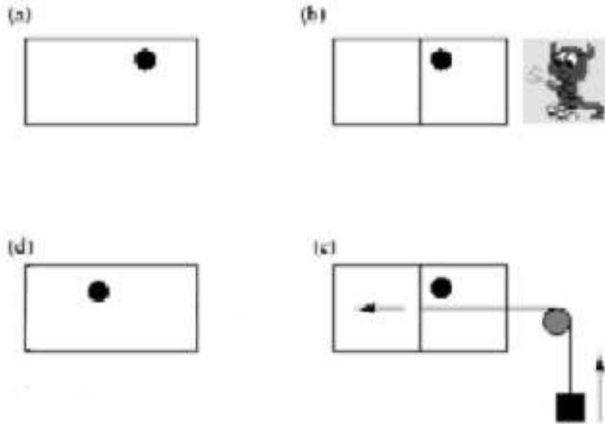
Figure 7: Szilard's demon engine.
