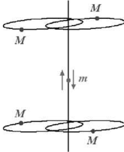
Figure 6: Xia's five body supertask.
