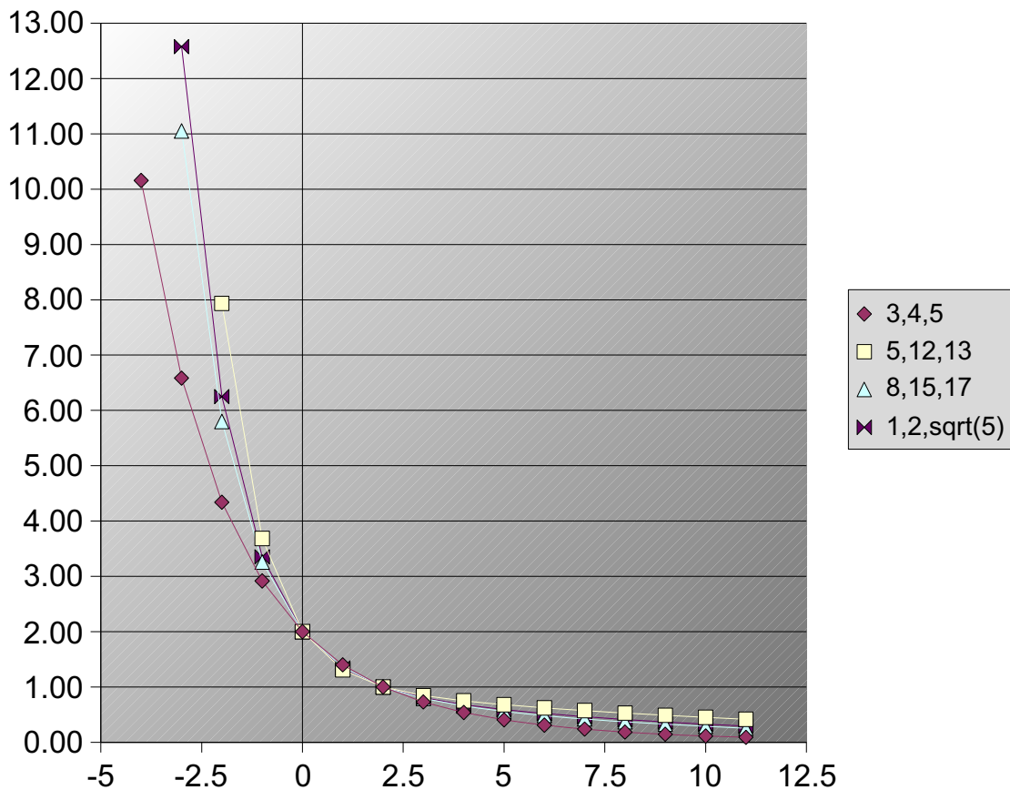
Numerical Test on Fermat's Theorem
