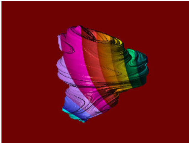
Picture 4. Random quaternion (Dofu-Zon)
