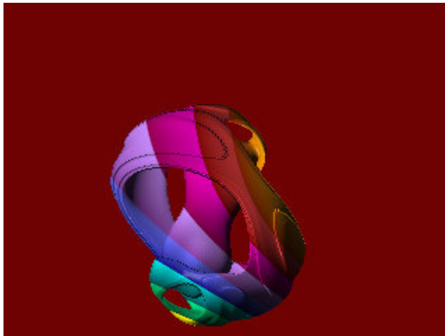
Picture 5. Random quaternion (Dofu-Zon)
