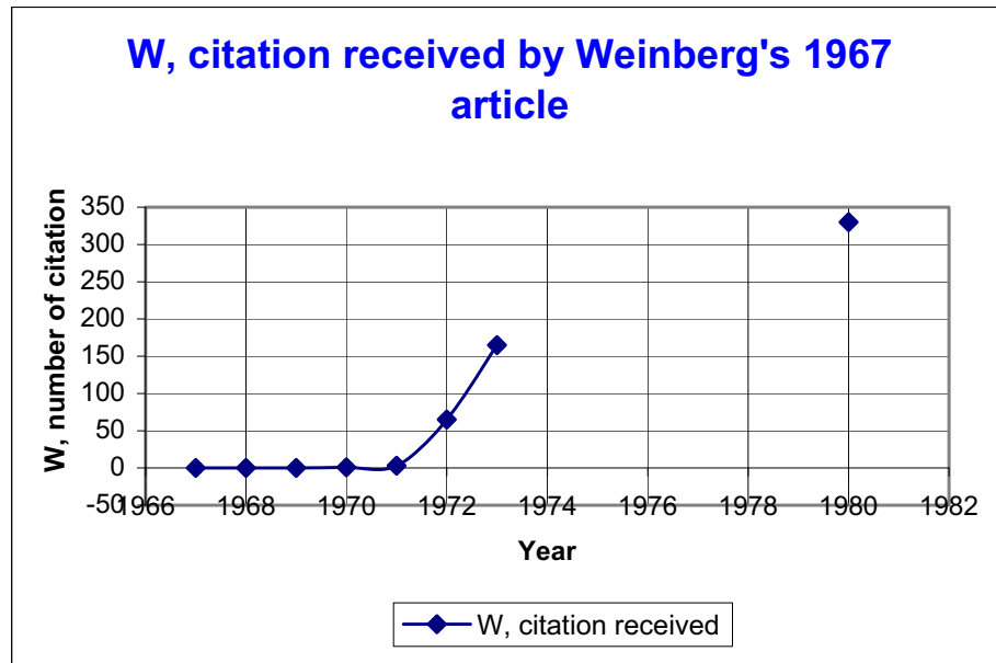
Graph 1. Graph plot of citation received by Weinberg's 1967
