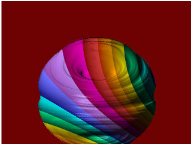
Picture 3. Random quaternion (Dofu-Zon)
