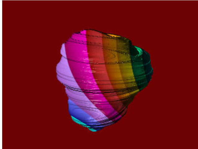
Picture 1. Random quaternion (Dofu-Zon)
