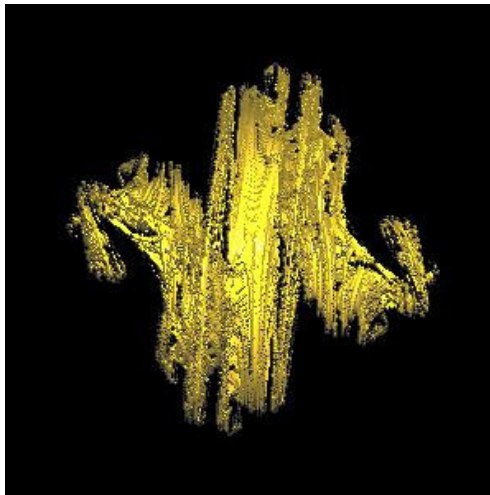
Picture 6. Quaternion, Q*Q*Q*Q+Q' (Fractal Explorer)
