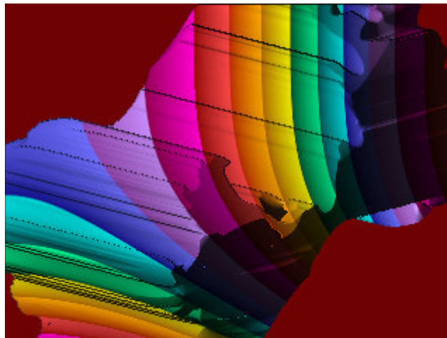
Picture 2. Random quaternion (Dofu-Zon)
