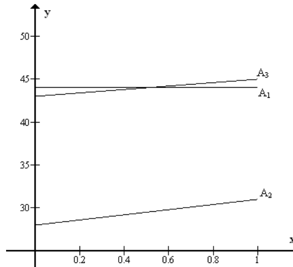
Figure 3. Alternatives' neutrosophic scores
