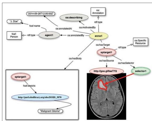
Figure 1: Using the Open Annotation (OA) model to annotate a magnetic resonance image depicting the brain of a pediatric patient with a diffuse glioma. The OA model provides tools for recording provenance, identifying portions of the annotated image, and encoding the list of statements about the annotated target. Source: http://www.sop.inria.fr/asclepios/projects/Health-e-Child/DiseaseModels/content/brain/TumorGrowth6_slowlygrowingpathologies.html
