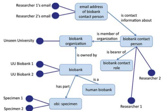
Figure 3: Central ontologized minimum information about biobank data sharing classes (from http://www.jbiomedsem.com/content/4/1/23/figure/F1 )
