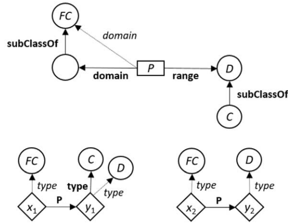
Fig. 1. Tbox of \mathbf{p3} and Abox of instance and non-instance of \exists P.C .
