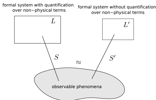
Figure 1: The platonistic physical theory and the nominalized physical theory should be equivalent on the empirical level.
