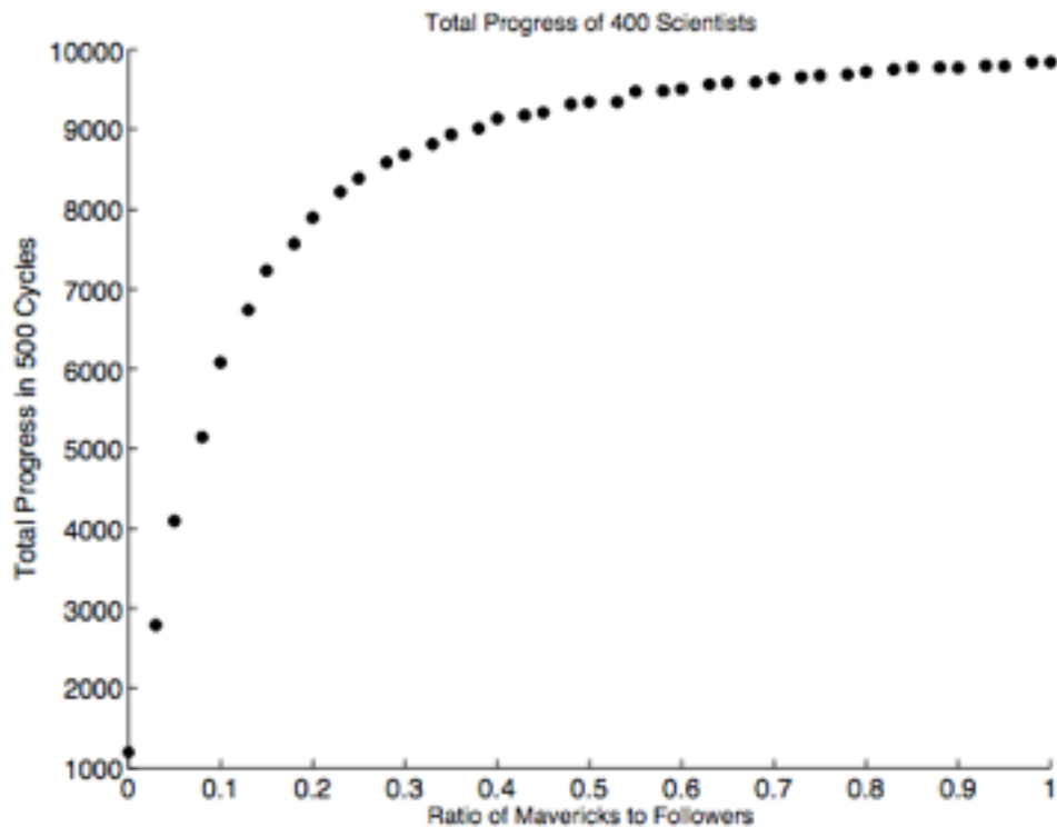
Figure 2: Total progress of different populations of 400 scientists after 500 rounds
