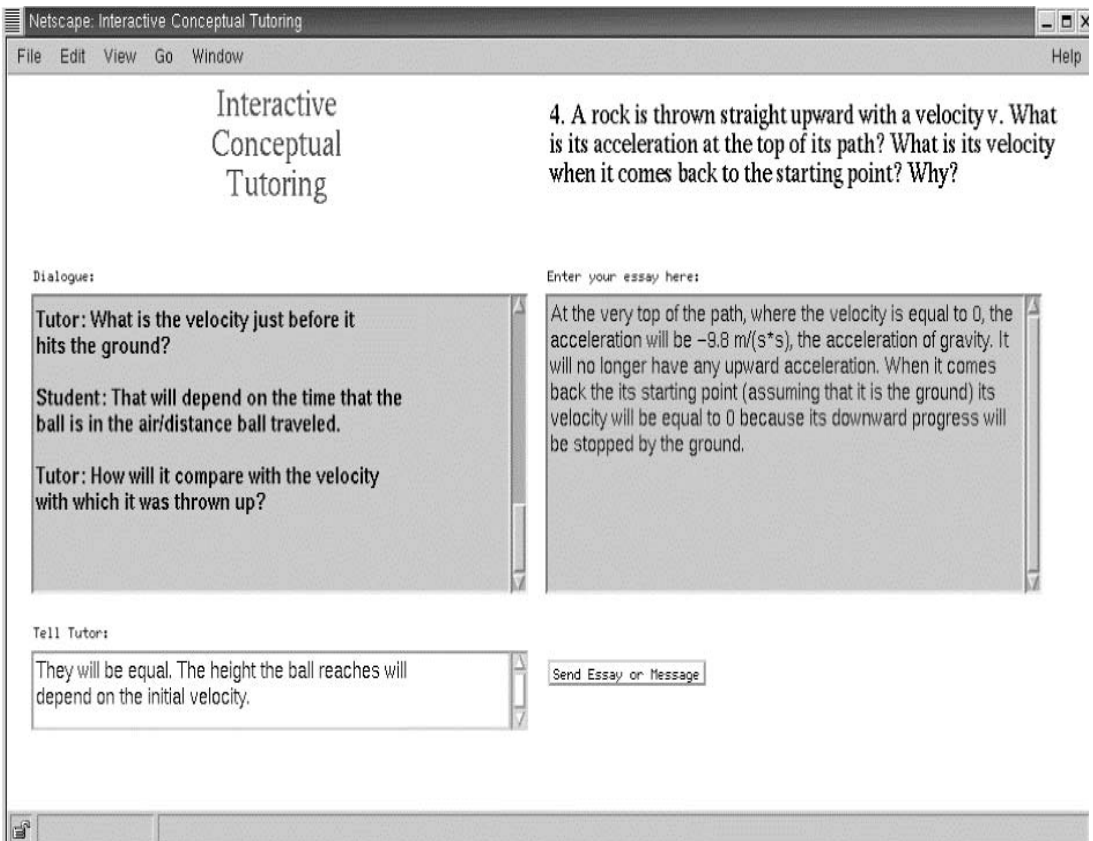
Fig. 1. User interface.
