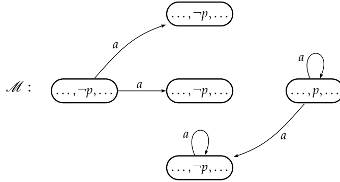
Figure 4.2: Dependence-based condition: preservation of literal \neg p under hypothesis a \not\rightarrow p .
