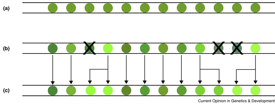
Fig. 2 “Ecological scaffolding in a droplet-based evolution machine ensures droplets are units of selection. Parallel horizontal lines are walls of Teflon tubes containing an emulsion of oil and regularly spaced droplets harbouring bacterial cells. a At the start of operation all droplets are founded by identical types. b A period of cellular growth occurs within droplets. During this stage mutations within individual cells arise that affect the colour of each droplet. Droplets whose colour is not sufficiently bright are marked for extinction allowing the possibility that when the contents of the droplets are
