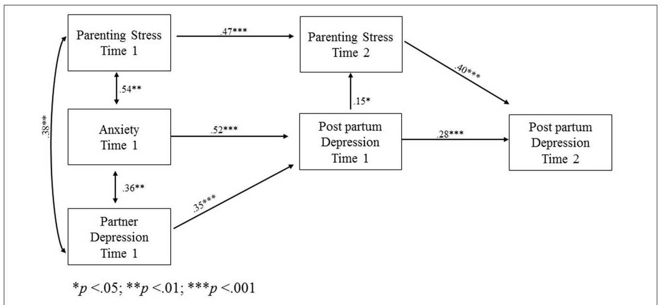
FIGURE 2 | Path model with statistically significant beta standardized coefficients for fathers.
