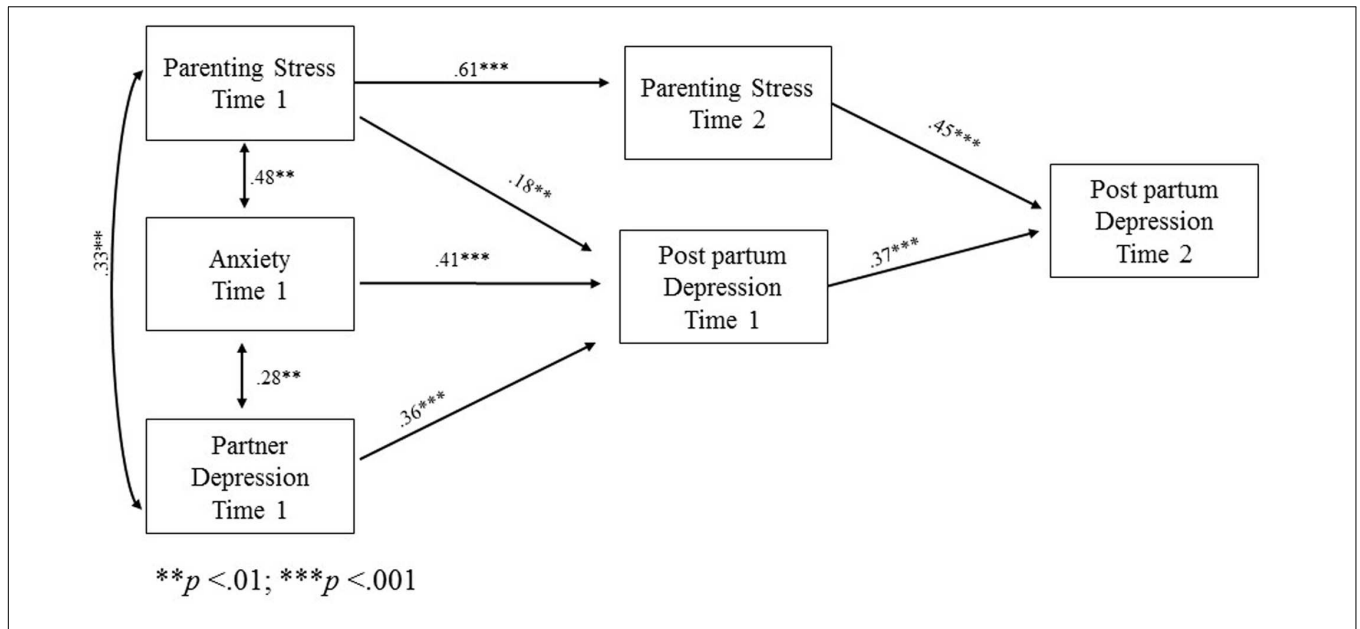
FIGURE 1 | Path model with statistically significant beta standardized coefficients for mothers.
