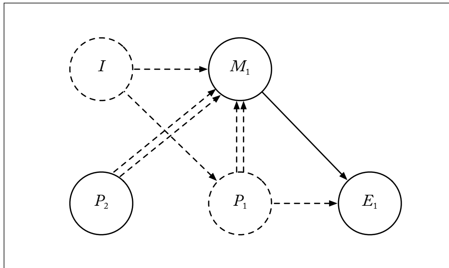
Figure 5: Diagram for \mathcal{M}_{PM_2} .
