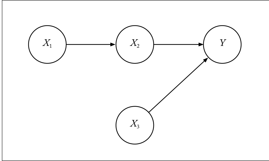
Figure 1: Diagram for \mathcal{M}_1 .
