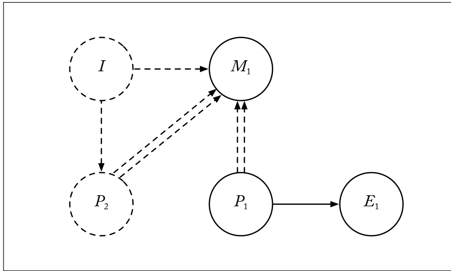
Figure 4: Diagram for \mathcal{M}_{PM_1} .
