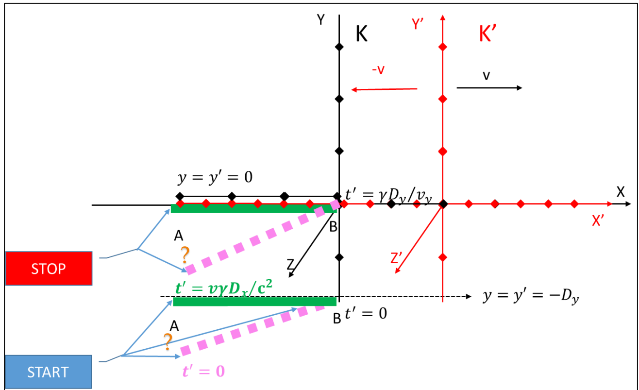
Figure 1 Transverse motion of the rigid rod
