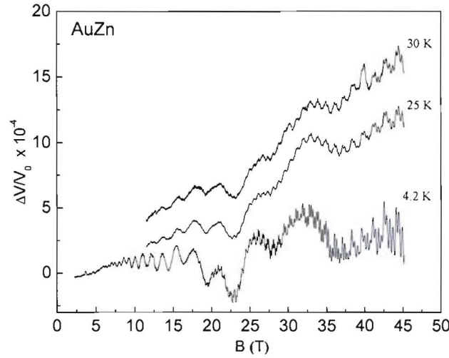
Figure 2. The oscillations of the speed of sound of AuZn measured at several temperatures in the martensitic phase. [After J.C. Lashley et al. (2007).]
