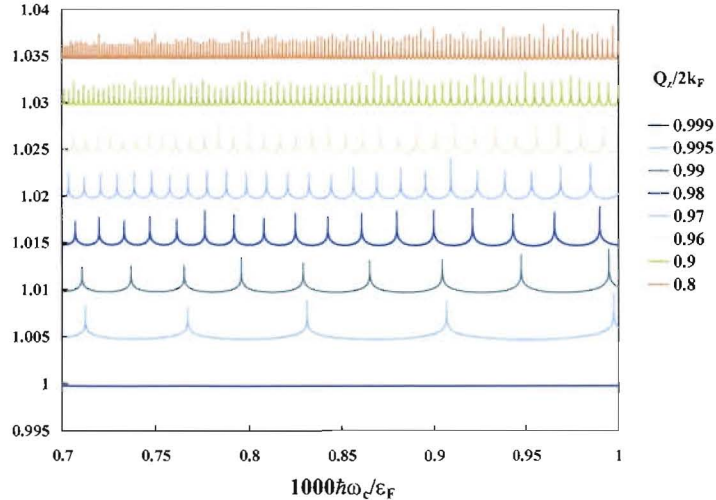
Figure 1. The oscillations of the normalized Lindhard function \chi_H(Q_z)/\chi_0(Q_z) with the magnetic field directed parallel to \underline{Q} . For clarity, the response is normalized to the H = 0 value and then is lowered by 0.005 for successively lower values of Q_z/2k_F . The curves are limited by the resolution of the plotting program.
