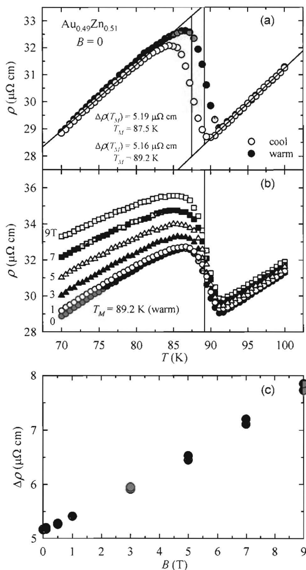
Figure 3. The temperature-dependence of the resistivity anomaly at the martensitic transition of the slightly off-stoichiometric compound \text{Au}_{0.49}\text{Zn}_{0.51} showing the thermal hysteresis (a), and for various applied magnetic fields (b). The field-dependence of the resistivity change at the martensitic transition of \text{AuZn} , for various applied fields (c).
