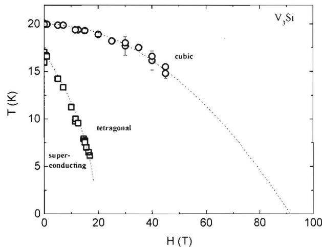
Figure 4. The field-dependence of the martensitic (cubic to tetragonal) phase transition and superconducting temperatures in V_3Si . [After P. A. Goddard et al. (2009).]
